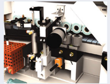
■ Pressure unit and edge cut device
