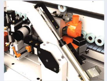
■ HF motor 12000 rpm / 0.3 kw / 200 Hz on twin blade of the end Trimming unit Twin blade tilting fixed at 0° and 15°
