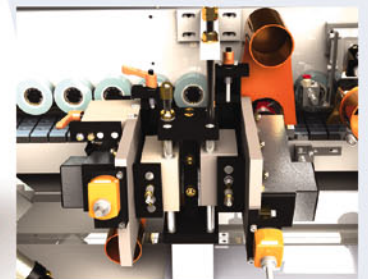
■ HF motor 12000 rpm / 0.3 kw / 200 Hz for up and down edge trimming unit
